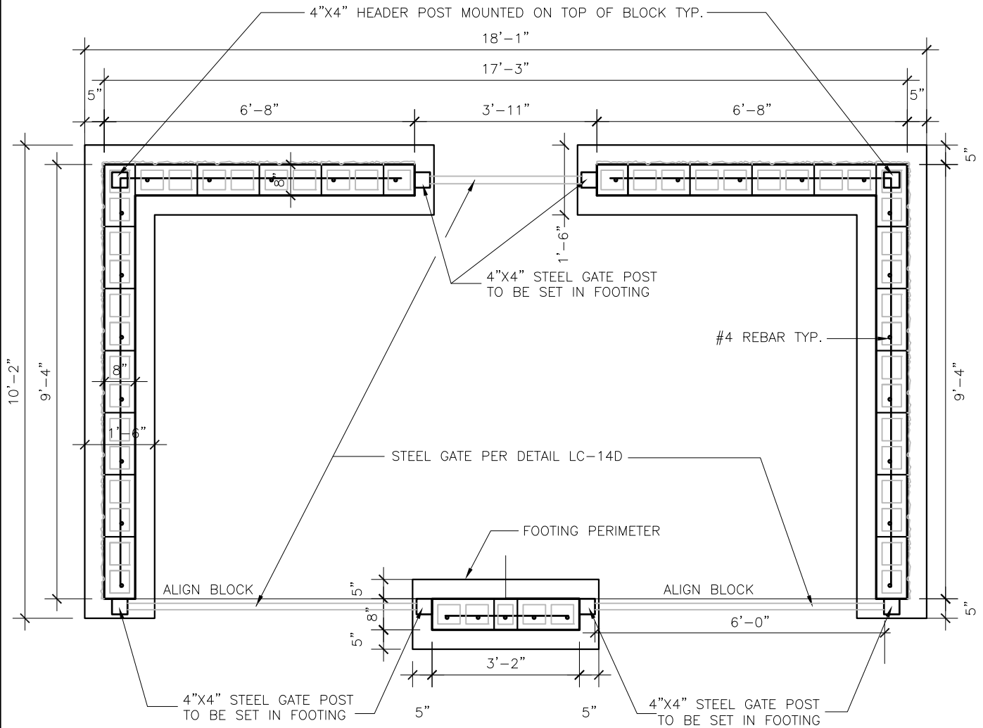
TRASH ENCLOSURE FOOTING LAYOUT
